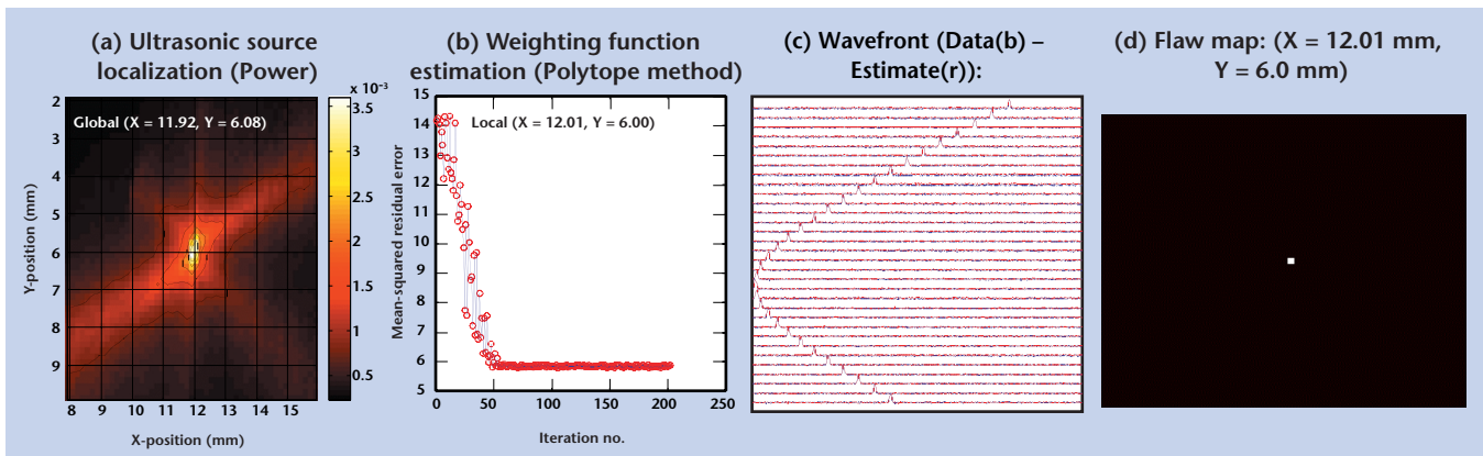
Figure 2. Application of flaw localization and mapping algorithms using T/R processing. Shown are (a) global (ultrasonic source localization), and (b) local (weighting-function estimation) search results for a synthesized aluminum slab. The wavefront match (c) and the final flaw map for a single flaw (d) are also shown.
