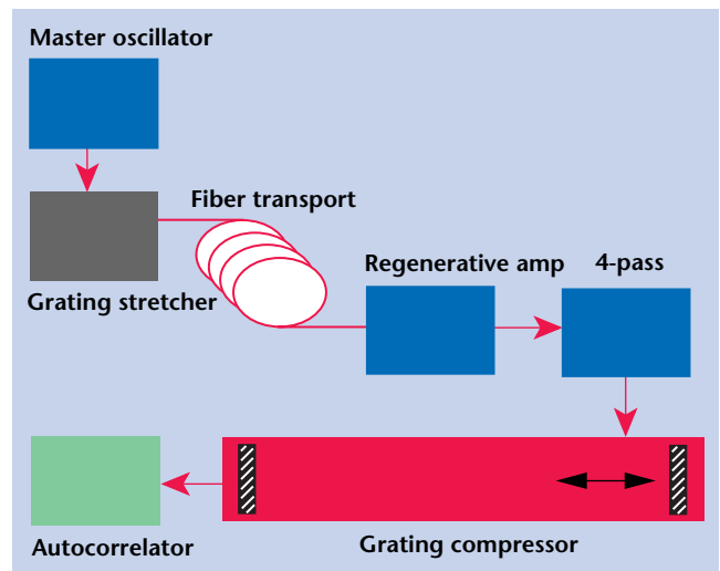
Figure 2. Block layout of the Falcon/Photoinjector laser showing major subsystems.
